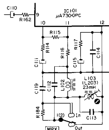
Fig. 7.2 3. MPX Filter
